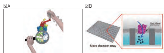
■回転分子モーターF1-ATPaseを1分子単位で力学操作し、分子の応答を探る Single-molecule manipulation of F1-ATPase rotary motor protein to elucidate the chemomechanical coupling mechanism. ■人工脂質膜チャンパーアレイ(左)と膜タンパク質1分子計測(右) Lipid bilayer chamber array (left) and single analysis of transporting activity of a membrane protein
